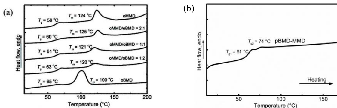
Figure 4: Thermal properties of (a) oBMD, oMMD and blends of oBMD/oMMD in mass ratios of 2:1; 1:1; 1:2; (b) pBMD-MMD.
