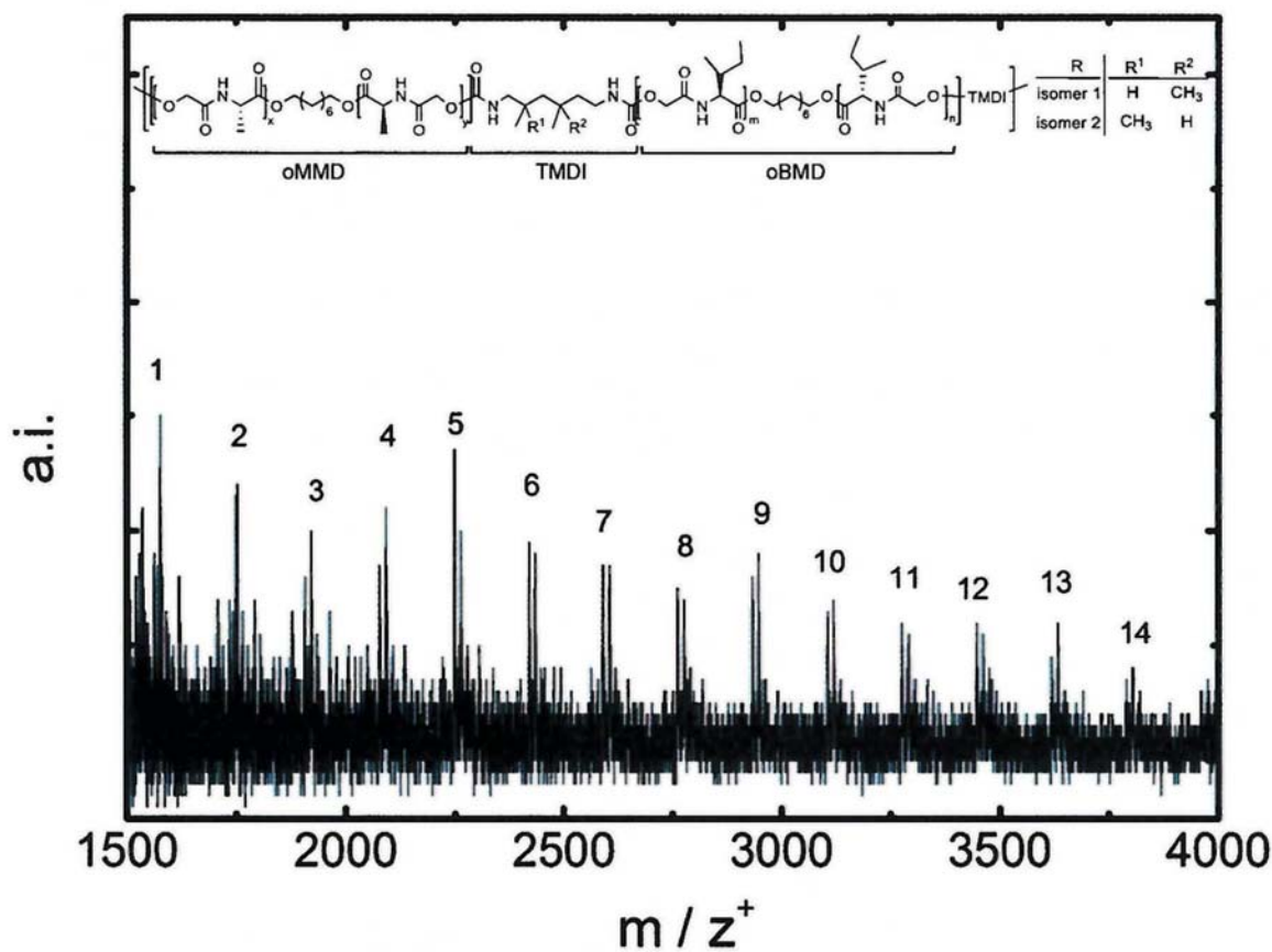
Figure 2: MALDI-TOF spectrum of pBMD-MMD.
