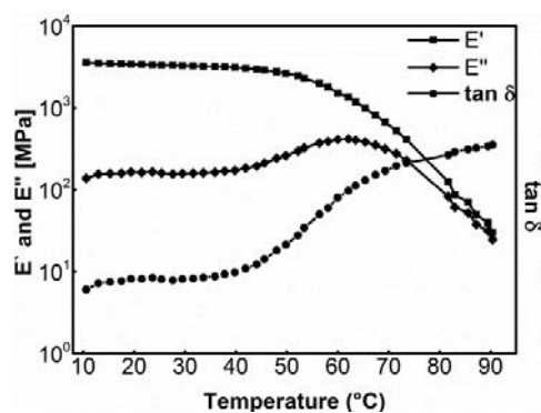
Figure 5. Thermomechanical properties of pBMD-MMD. E' : Storage Modulus, E'' : Loss Modulus, \delta : Phase Angle.
