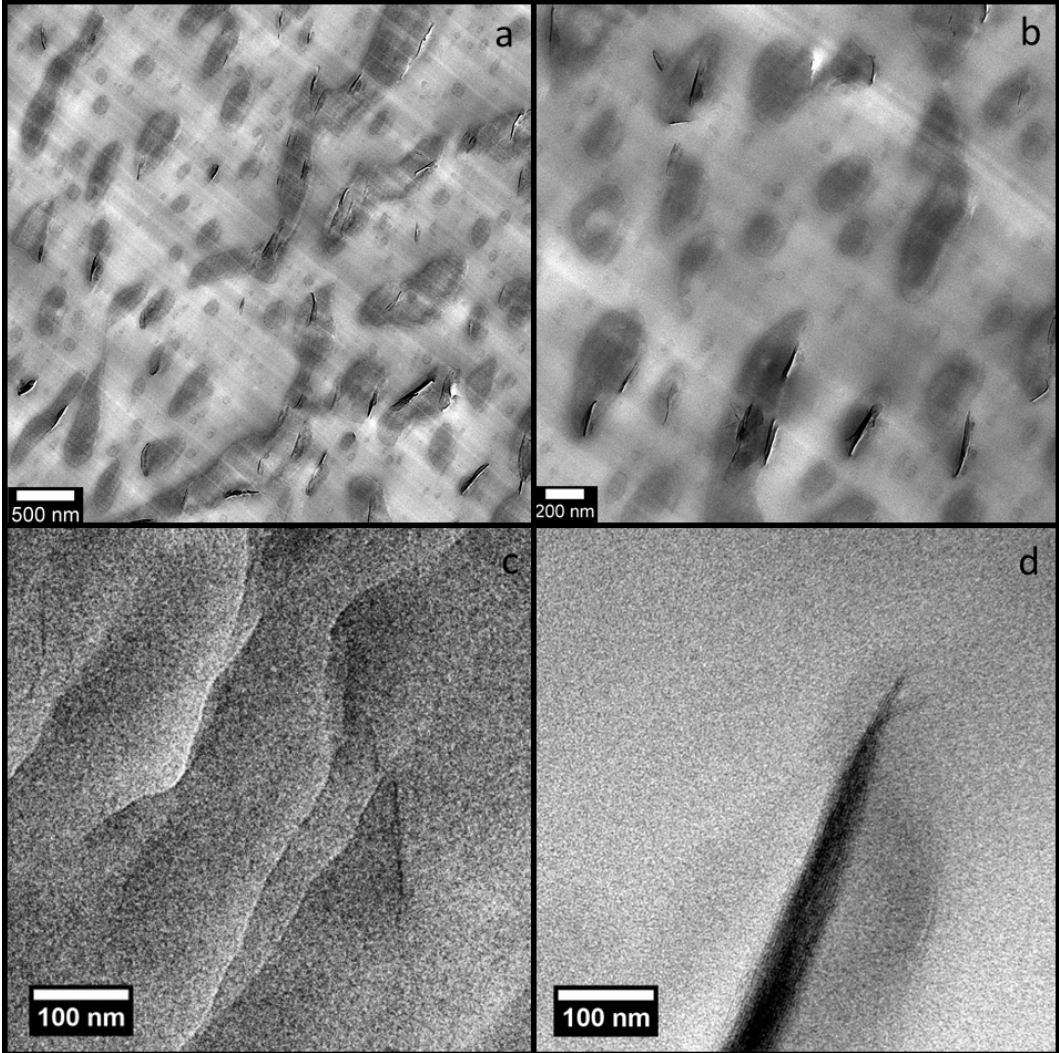
Figure 1. TEM images of HPC/SAN 7/3 1wt% MB30B at different magnifications
