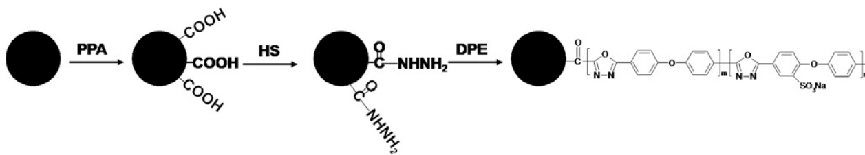
Figure 1. Proposed route for the oxidation of the CB represented as a black circle and grafting of POD on its surface.
