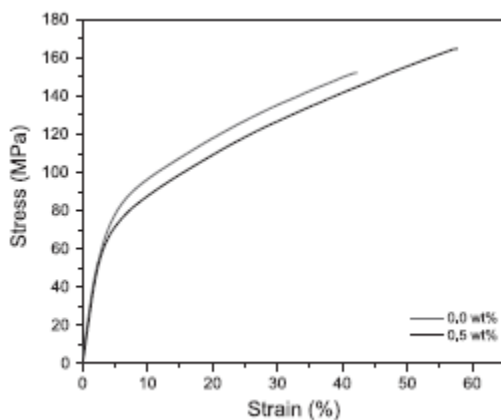
Figure 6. Representative stress-strain curves of the of the CB/POD nanocomposites.
