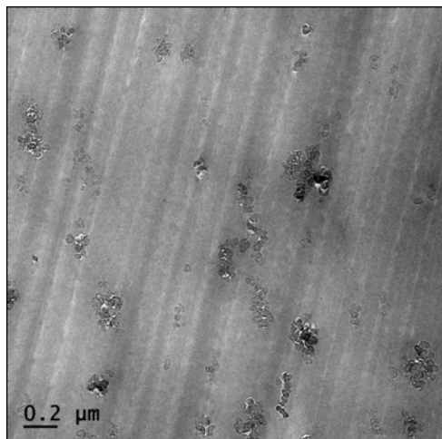
Figure 8. TEM image of the fracture surface of the POD nanocomposites reinforced with 0.5 wt% of CB after conducting tensile tests.
