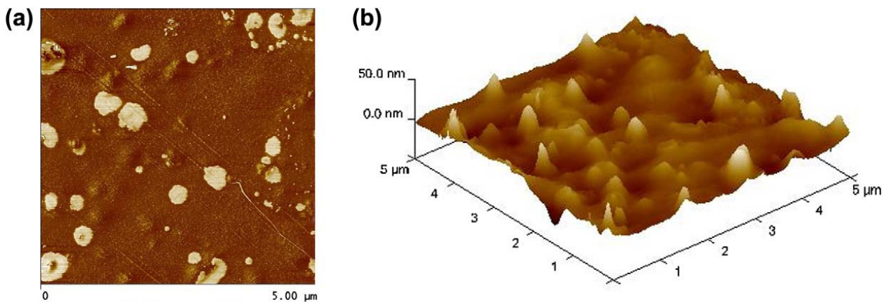
Figure 7. AFM images of the fracture surface of the POD nanocomposites reinforced with 0.5 wt% of CB after conducting tensile tests.
