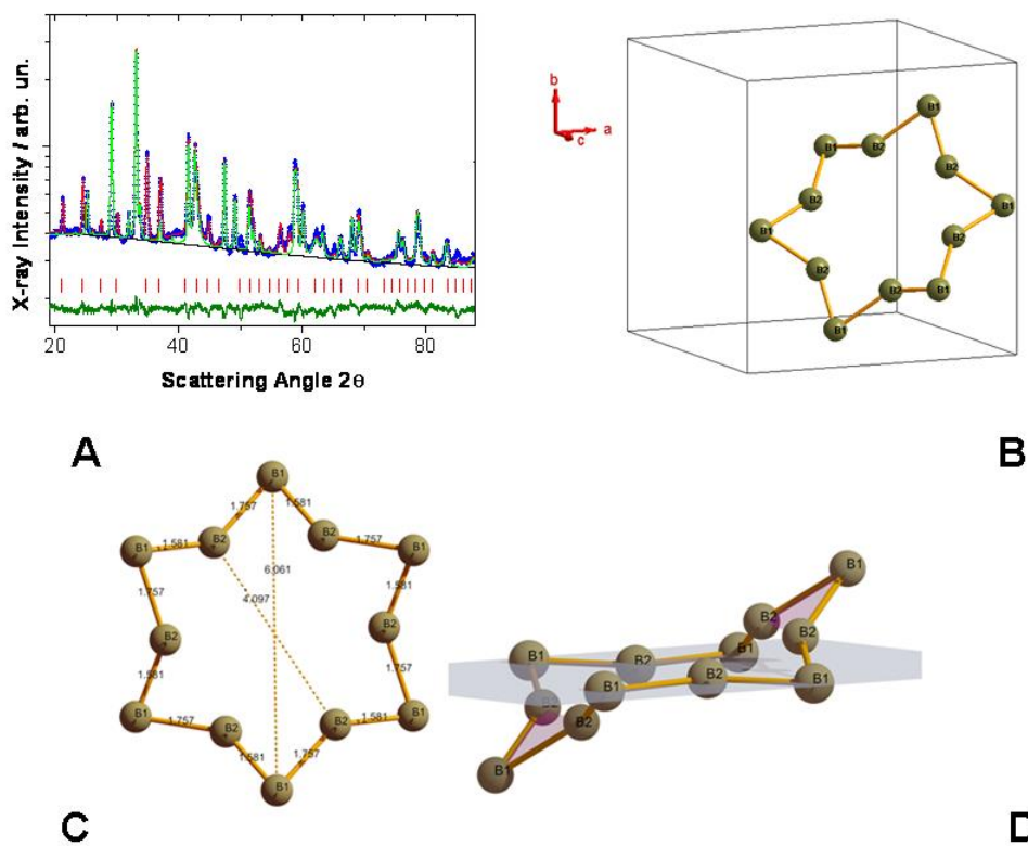
Fig. 3 A: Rietveld fit to the total experimental pattern (dots) including the contribution of the proposed Pa-3 cubic (continuous line). Peak positions and residuals are shown in the bottom. B: sketch of the B-atoms position in the unary cell, a cycle of twelve boron atoms C: alternating B-B bond length of 1.58 Å and 1.76 Å. D: Six of twelve atoms of the interconnected B-atoms lie on a plane.
